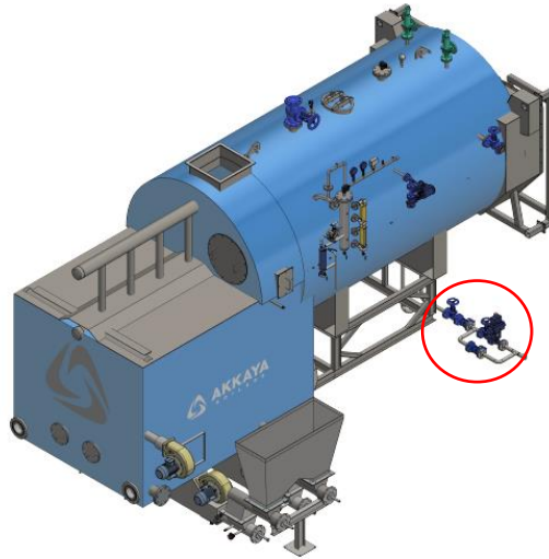
Figure Ap. 4.3.1 Bottom Blowdown Valve
