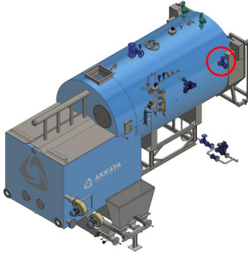
Figure Ap. 4.6.1 Boiler Water Inlet Valve & Check Valve
