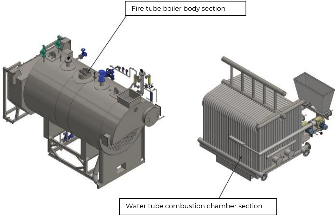
Figure 2.3.1 YHYB Boiler Main Parts
