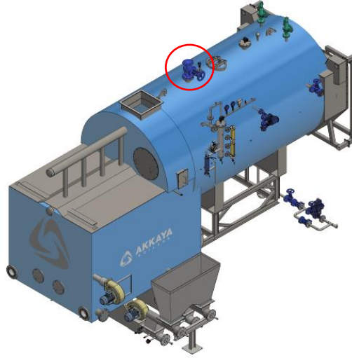
Figure Ap. 4.2 Steam Exit Valve Position on The Boiler
