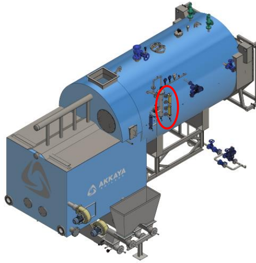
Figure Ap. 4.9 Reflex Glass Boiler Water Level Indicator
