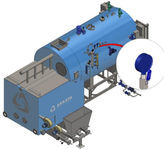
Figure Ap. 4.12 Manometer & Manometer Valves
