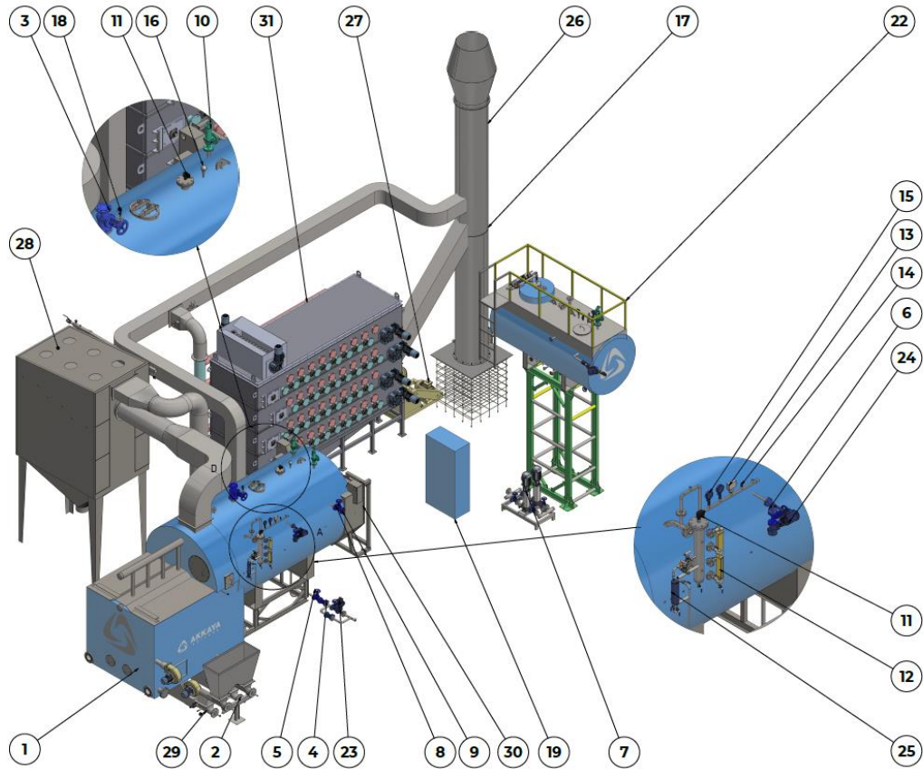
Figure 4 Sample Boiler Accessories & Auxiliaries
