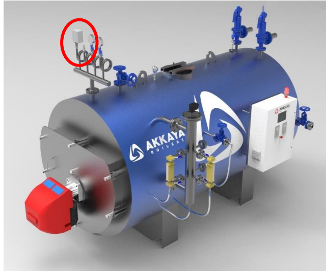
Figure Ap. 4.10 Pressure Switches
