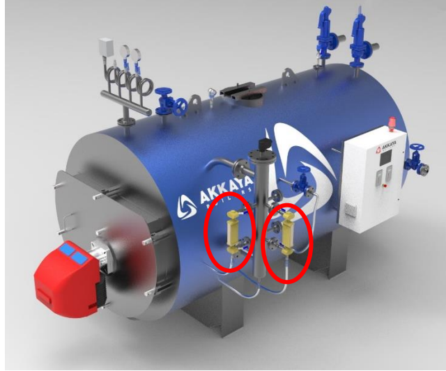
Figure Ap. 4.9 Reflex Glass Boiler Water Level Indicator
