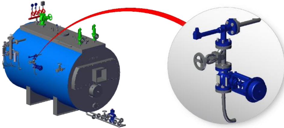
Figure Ap.4.4.2 Automatic Surface Blowdown System
