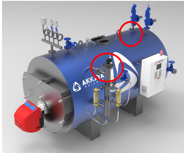
Figure Ap.4.8.1 Boiler Automatic Water Level Controller
